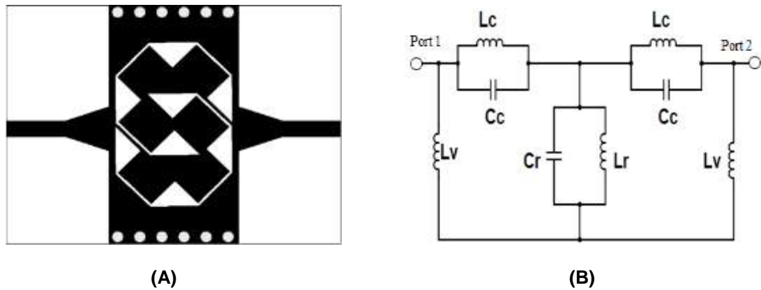
Figure 10. Configuration of the SIW bandpass filter loaded by proposed CSRR (A). Equivalent circuit of the SIW bandpass filter loaded by CSRR nested configuration (B) (Lumped-element values are C_r = 6.1 pF, L_r = 4.15 nH, C_c = 1.55 pF, L_c = 1.7 nH, L_v = 1.95 nH).
