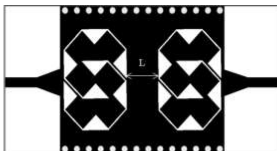
Figure 17. Layout of the proposed two-stage SIW bandpass filters loaded by proposed CSRR.
