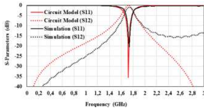
Figure 11. EM-simulated and circuit model S-parameters of SIW bandpass filter loaded by CSRR.
