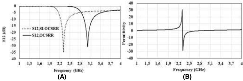
Figure 2. Simulated transmission responses of OCSRR and SI-OCSRR (A). Real part of the negative permittivity of the proposed CSRR (B).
