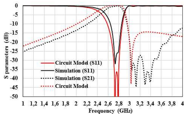
Figure 7. EM-simulated and circuit model S-parameters of SIW bandpass filter loaded by SI-OCSRR reversely side by side configuration. (The geometrical parameters are w = 8.3\text{ mm} , l = 15.8\text{ mm} , d = 0.8\text{ mm} , P = 1.5\text{ mm} , d_1 = 0.86\text{ mm} , d_2 = 0.23\text{ mm} ).
