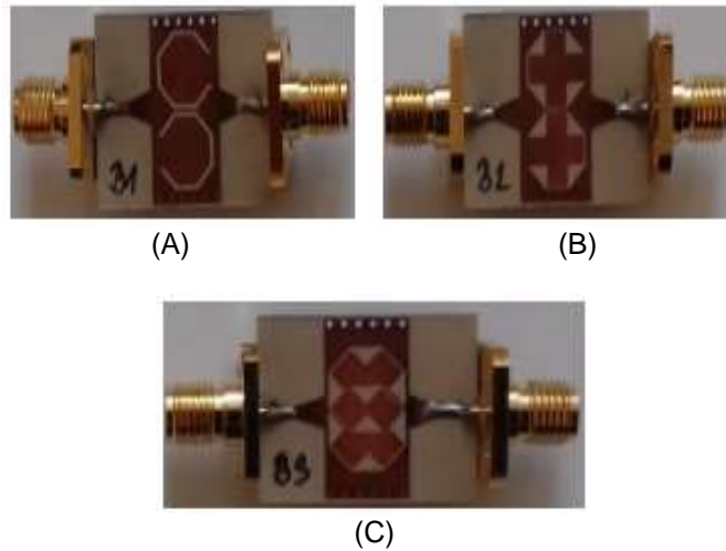
Figure 13. Photograph of the fabricated SIW bandpass filters loaded by (A) classical CSRR (B) proposed CSRR (Type I), (C) proposed CSRR (Type II).
