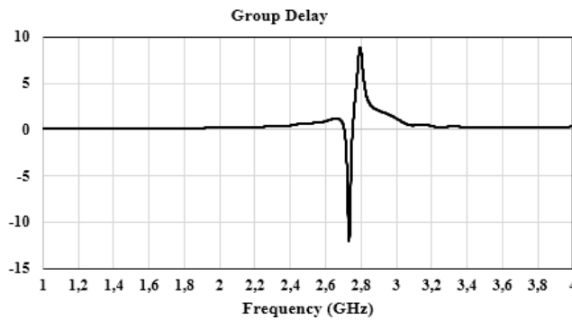
Figure 9. Group delay of the filter loaded by SI-OCSRR (Type I)
