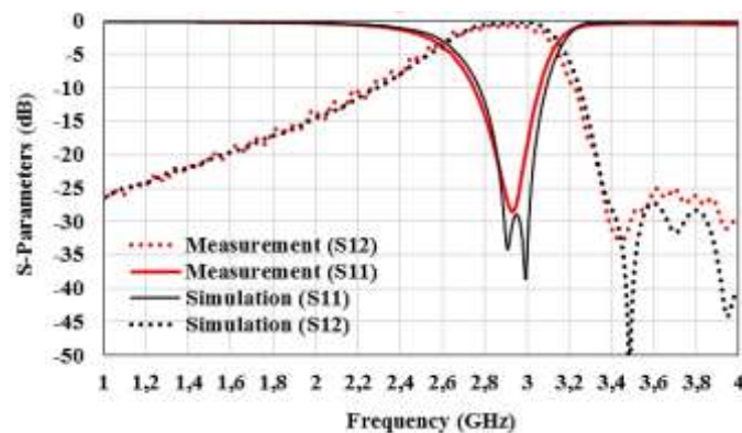
Figure 14. Simulated and measured frequency responses of the SIW filters bandpass loaded by the classical CSRR.
