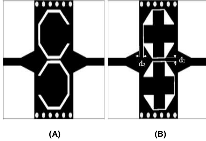
Figure 4. Configuration of the SIW bandpass filter loaded by (A) the classical octagonal CSRR, (B) the proposed octagonal CSRR.
