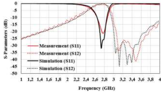
Figure 15. Simulated and measured frequency responses of the SIW bandpass filters loaded by the proposed CSRR with side by side reversely configuration.
