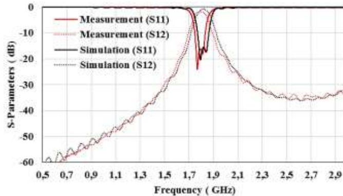
Figure 19. Simulated and measured frequency responses of the tow stage SIW bandpass filters loaded by the proposed CSRR with nested configuration.
