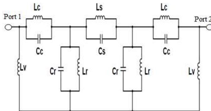
Figure 5. Equivalent circuit of the SIW bandpass filter loaded by CSRR side- by- side reversely configuration, (Lumped-element values are L_v = 3.6 nH, C_r = 4.95 pF, L_r = 0.95 nH, C_c = 0.65 pF, L_c = 0.35 nH, L_s = 0.49 nH, C_s = 5.37 pF).
