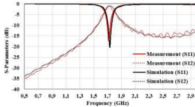
Figure 16. Simulated and measured frequency responses of the SIW bandpass filters loaded by the proposed CSRR with nested configuration.
