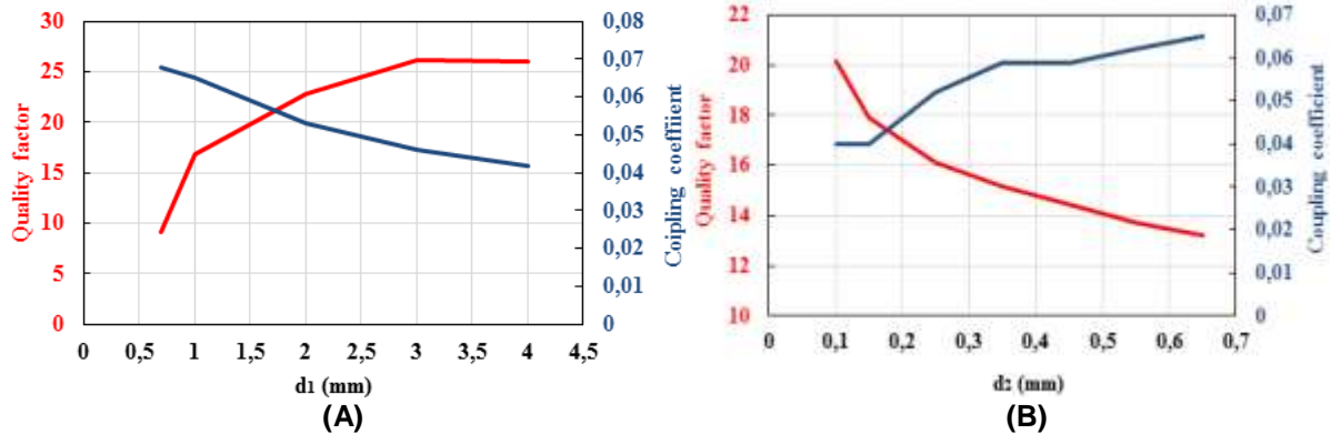
Figure 6. External quality factor and coupling coefficient versus distance d_1 (A). External quality factor and coupling coefficient versus distance d_2 (B).
