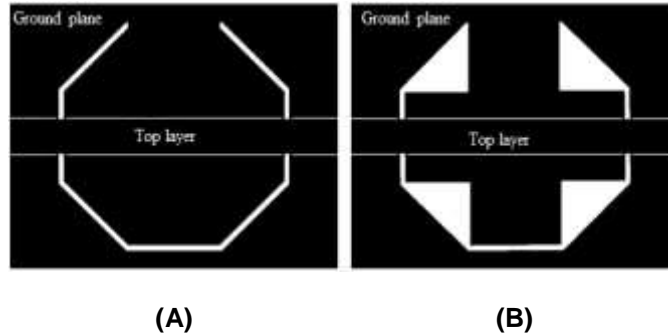
Figure 1. Micro-strip TL loaded with, (A) conventional OCSRR, (B) SI- OCSRR.
