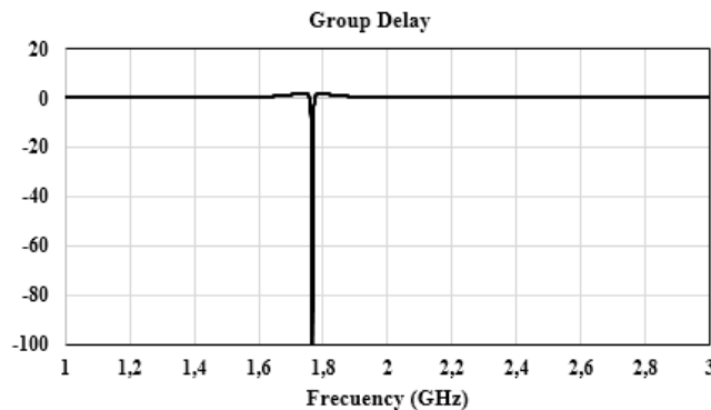
Figure 12. Group delay of the proposed filter loaded by SI-OCSRR (Type II)
