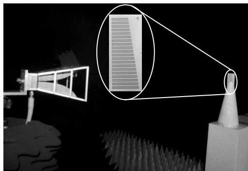
Fig. 1. Measurement setup using monostatic configuration with the detail of the original 20-bit tag.
