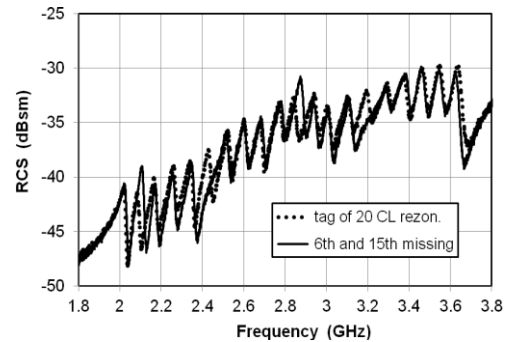
Fig. 9 Measured RCS response of 20-bit chipless tags using rearranged half-spiral capacitive loaded dipoles, representing bit words '11111111111111111111', and '11111011111111011111'.
