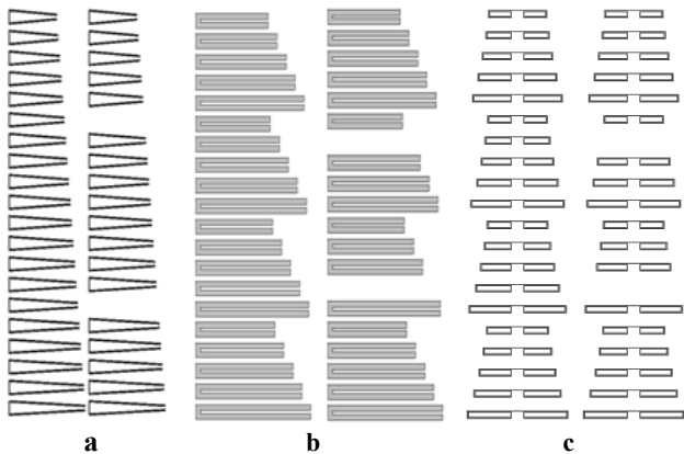
Fig. 6 Layouts of investigated modifications of folded-dipole scatterers: a) arrays of 20 T-UDs [10], coding information 11111111111111111111, and 11111011111111011111 by missing 6 th and 15 th elements, b) rearranged resonators in the array [9] coding the same information, c) half spiral capacitive loaded dipoles [12].
