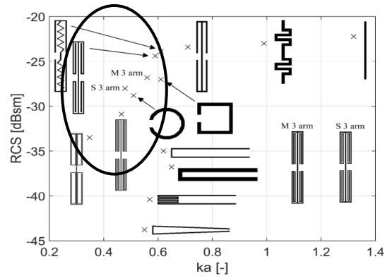
Fig. 5 Comparison of scatterers according the RCS and ka product.
