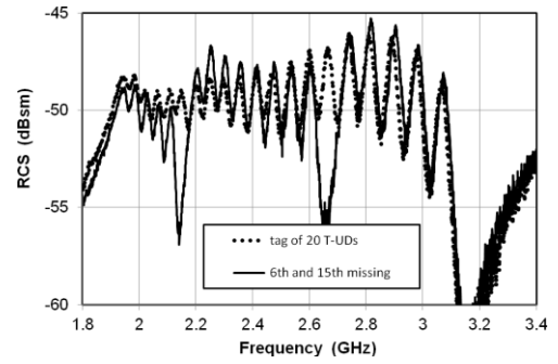
Fig. 7 Measured RCS response of 20-element tags composed of tapered U-folded dipoles, and tag coded by missing 6 th and 15 th elements, [11].
