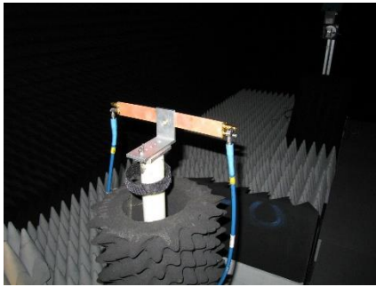
Fig. 6. Measurement of the radiation patterns of the fabricated antenna in the anechoic chamber.
