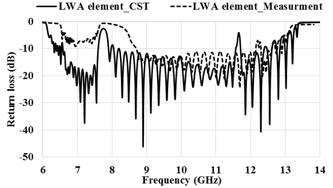
Fig. 4. Measured and simulated S11 of the first CRLH SIW leaky wave antenna
