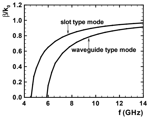
Fig.17 Normalized phase constant of the even dominant slot type mode, and waveguide type mode on a shielded conductor-backed slotline, ⑬ in Fig. 1, when slot width w=20 mm, height of the shield 2h=4 mm, its width b=50 mm and permittivity \epsilon_r=1 .
