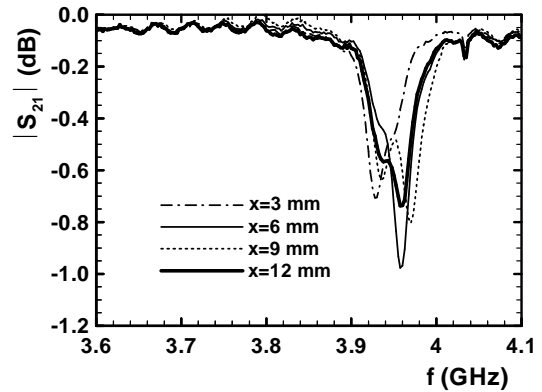
Fig. 9 Measured transmission of the R32 waveguide with two particles in dependence on lateral shift x defined in Fig. 5, for y = 0 mm.
