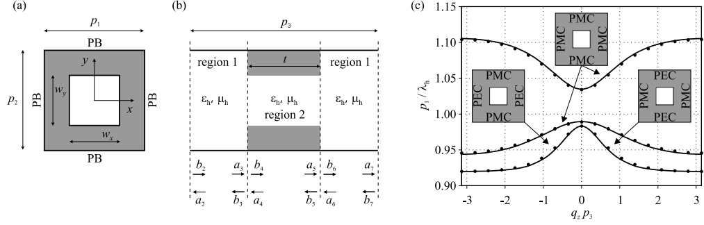
Fig. 1. Panels (a) and (b) show the front and side view of the analyzed unit cell. Panel (c) shows the dispersion diagram for normal incidence on a structure with p_1 = p_2 , w_x = w_y = p_1/3 , p_3 = p_1/9 , t = p_1/30 and some host material (lines come from the presented method, while dots come from CST). The lateral boundaries are indicated in all the panels and are either a periodic boundary (PB), a perfect magnetic conductor (PMC) or a perfect electric conductor (PEC). The gray regions in all the panels represent a perfect electric conductor.
