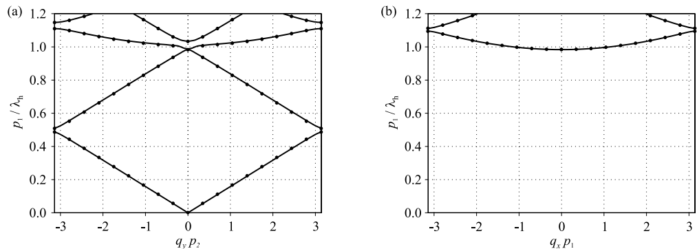
Fig. 2. Band diagram cut for q_z = q_x = 0 corresponding to the TM case (a) and band diagram for q_z = q_y = 0 corresponding to the TE case (b). The structural parameters are identical with Fig. 1c. The lines come from the presented method, while dots come from CST.
