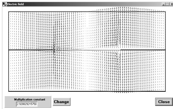
Fig. 17 Electric field of the even slot type dominant mode on the cross-sectional plane of the wide slotted line specified in Fig. 15 at f=7.5 GHz.
