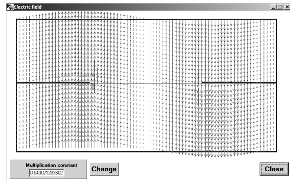
Fig. 18 Electric field of the even perturbed waveguide type mode on the cross-sectional plane of the wide slotted line specified in Fig. 15 at f=7.5 GHz.
