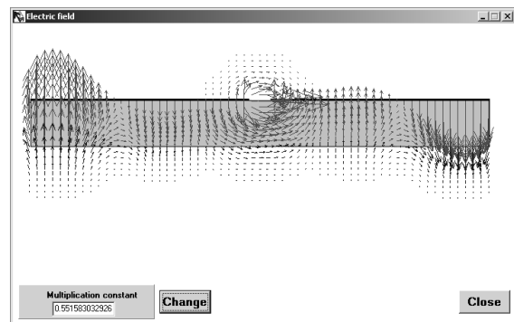
Fig. 10 Electric field of the even surface leaky mode on a slotline with w=5.65 mm, h=14.6 mm, \epsilon_r=2.6 and h/\lambda_0=0.4 .
