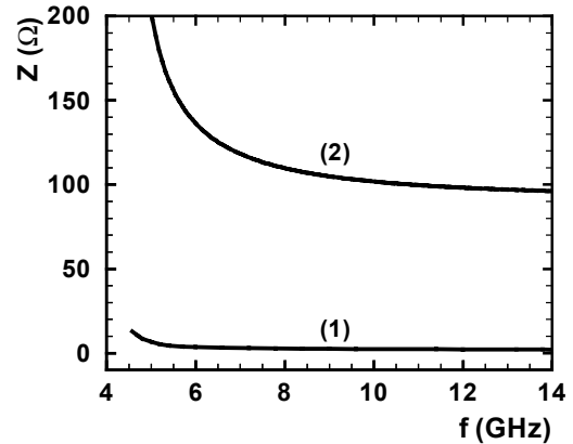
Fig. 16 The characteristic impedance (1) of the line specified in Fig. 15 with the slot type mode, and (2) of the line when w=1 mm, 2h=10 mm, b=23 mm, \epsilon_r=1 , on which the slot type mode propagates.
