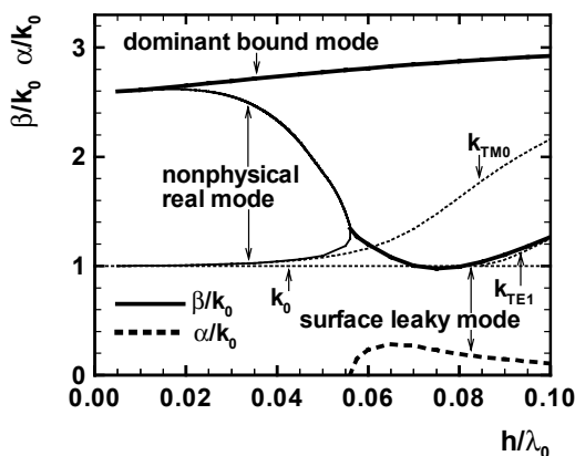
Fig. 3 Dispersion characteristics of the microstrip line, ① in Fig. 1, with strip width w=0.6 mm, substrate thickness h=0.635 mm and permittivity \epsilon_r=10 .
