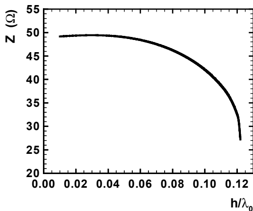
Fig. 13 Characteristic impedance of a coplanar waveguide specified in Fig. 12.
