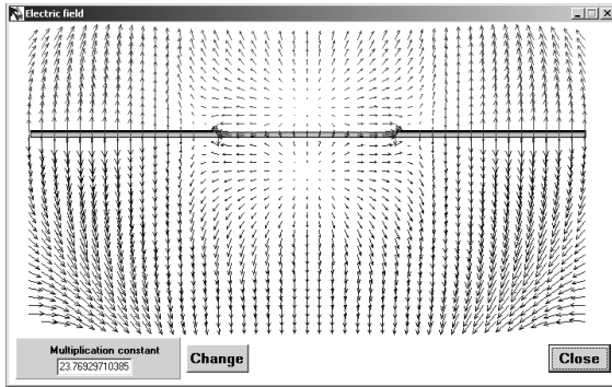
Fig. 11 Electric field of the odd 1st space leaky mode on the slotline specified in Fig. 6 at h/\lambda_0=0.012 .
