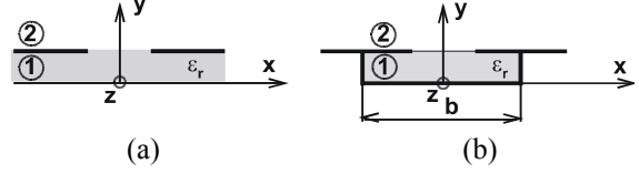
Fig. 2 Cross-section of a slotline (a) and conductor-backed slotline with the finite width of the substrate metallized on the side walls (b).
