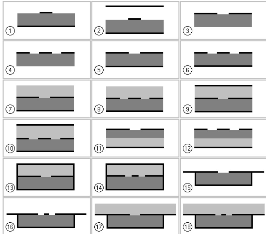
Fig. 1 Cross-sections of planar transmission lines analyzed by the APTL program.
