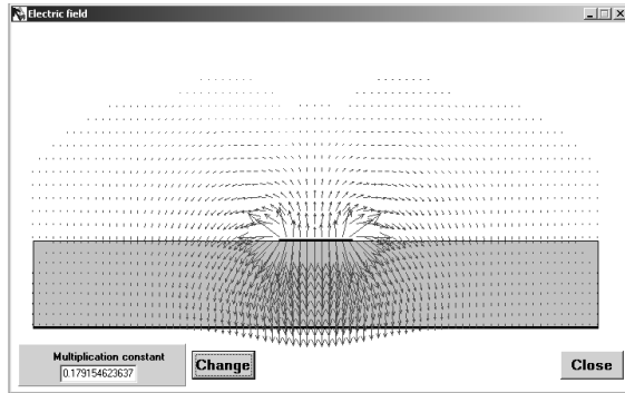
Fig. 5 Electric field of the dominant bound mode on the cross-sectional plane of the microstrip line, ① in Fig. 1, when w=1 mm, h=1 mm and \epsilon_r=2.2 .
