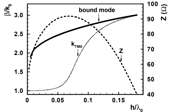
Fig. 8 Phase constant of the dominant bound mode and the characteristic impedance of a slotline, ③ in Fig. 1, with w=0.15 mm, h=0.625 mm and \epsilon_r=10.8 .
