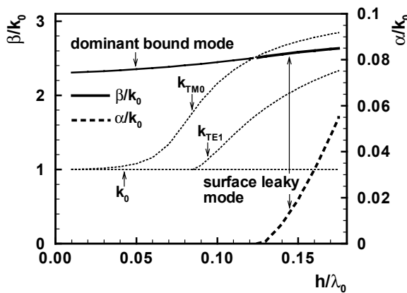
Fig. 12 Dispersion characteristics of a coplanar waveguide, \textcircled{4} in Fig. 1, when central strip width s=0.6 mm, slot width w=0.25 mm, substrate thickness h=1 mm and permittivity \epsilon_r=10 .
