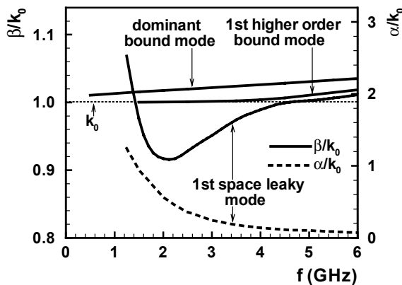
Fig. 6 Dispersion characteristics of a slotline, ③ in Fig. 1, with slot width w=60 mm, substrate thickness h=1.2 mm and permittivity \epsilon_r=2.6 .
