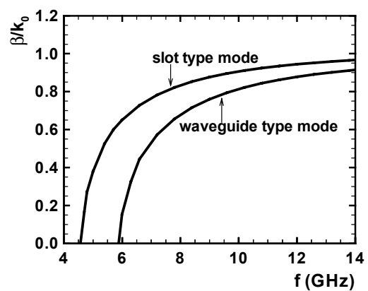
Fig. 15 Normalized phase constant of the even dominant slot type mode, and waveguide type mode on the shielded conductor-backed slotline, \textcircled{13} in Fig. 1, when slot width w=20 mm, height of the shield 2h=4 mm, its width b=50 mm and permittivity \epsilon_r=1 .
