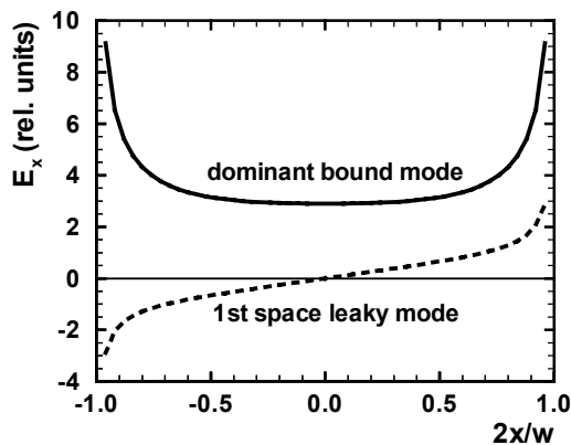
Fig. 7 Transversal electric field component within the slot of the slotline specified in Fig. 6 when h/\lambda_0=0.012 .
