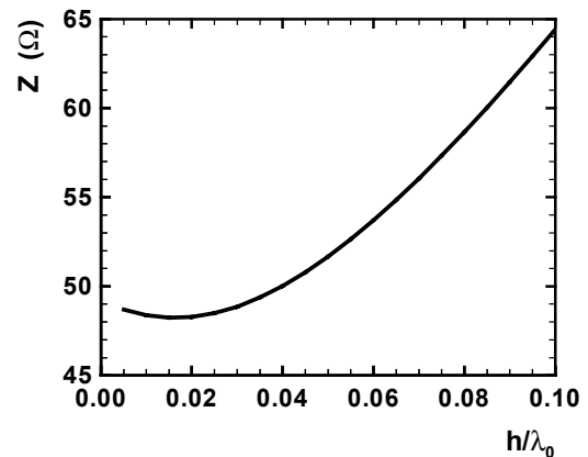
Fig. 4 The characteristic impedance of the microstrip line specified in Fig. 3.
