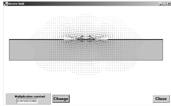
Fig. 14 Electric field of the dominant bound mode on the cross-sectional plane of the coplanar waveguide specified in Fig. 12.
