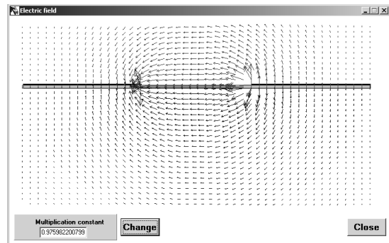
Fig. 9 Electric field of the even dominant bound mode on the slotline specified in Fig. 6 at h/\lambda_0=0.012 .
